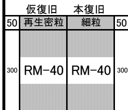
図7-2 歩道舗装(35)
